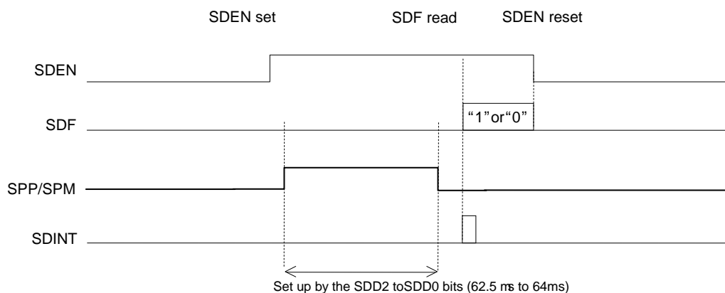
Figure 24-5 Example of Operation Timing
