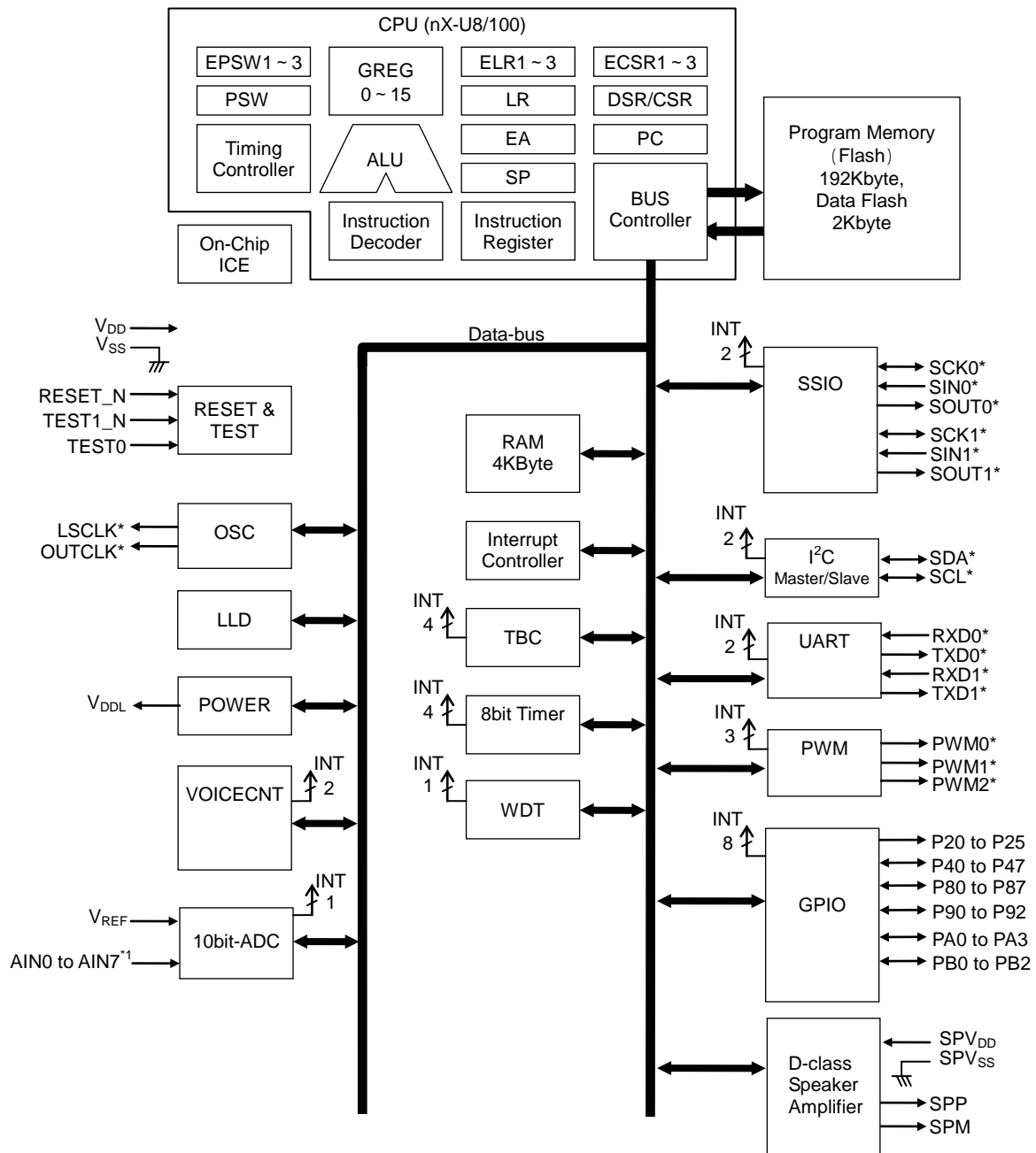
Figure 1-1 Block Diagram of ML610Q327
