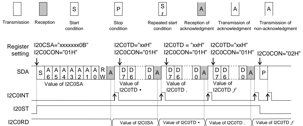
Figure 20-2 Operation Timing in Data Transmit (Write)
