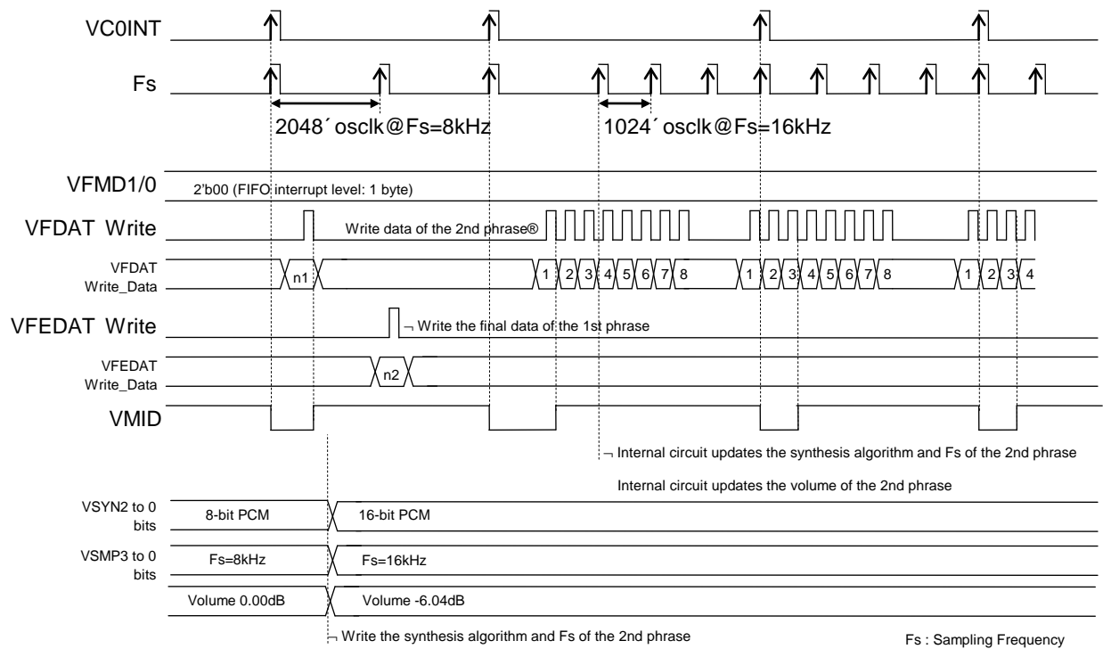
Figure 23-7 Operation Timing of Continuous Playback
