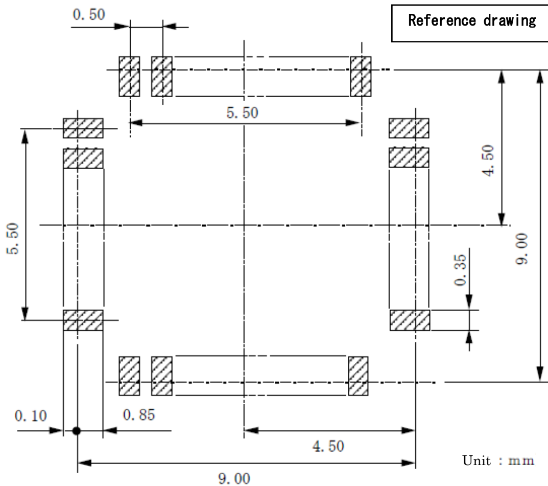
Figure of soldering department terminal existence range (48-pin TQFP)
