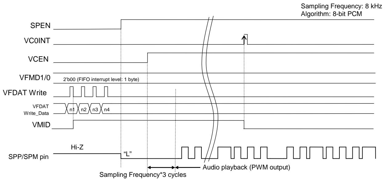
Figure 23-8 Power-Up Timing
