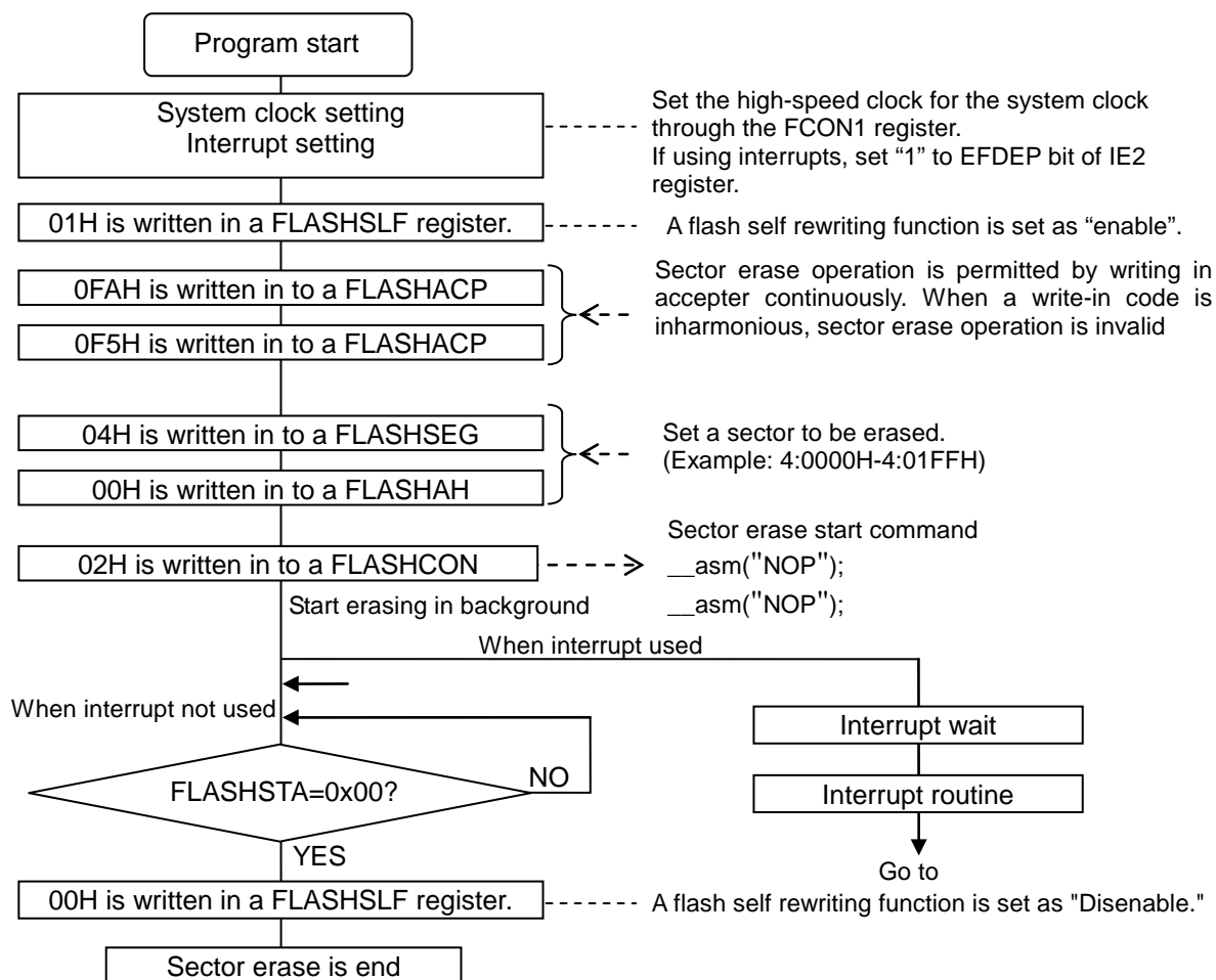
Figure 25-1 Sector erase flow
