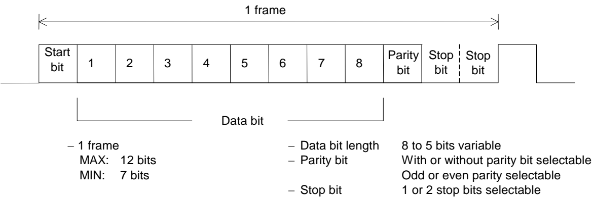
Figure 19-3 Negative Logic Input/Output Format
