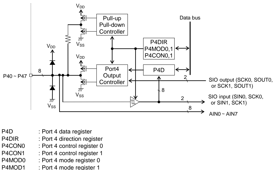
Figure 7-1 Configuration of Port 4
