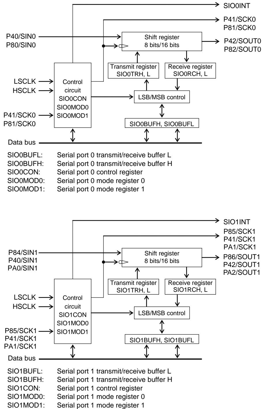
Figure 18-1 Configuration of Synchronous Serial Port 0 and 1
