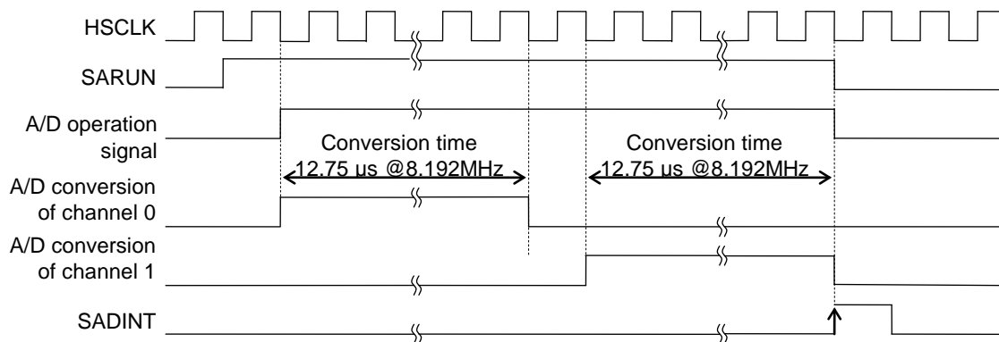
Figure 22-3 SA-ADC Operation Timing
