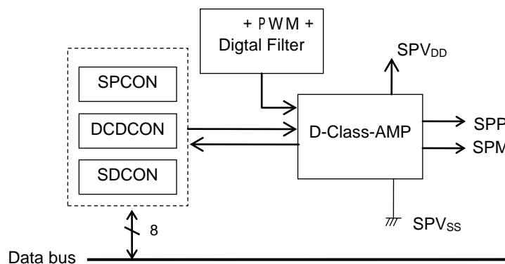
Figure 24-1 Speaker Amplifier Configuration
