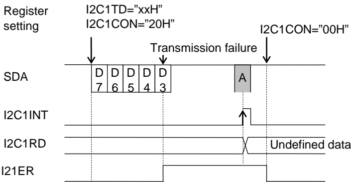
Figure 21-5 Operation Timing When Transmission Fails
