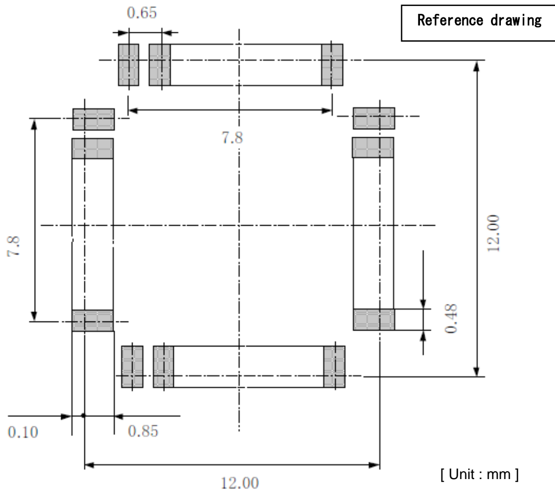
Figure of soldering department terminal existence range (52-pin TQFP)
