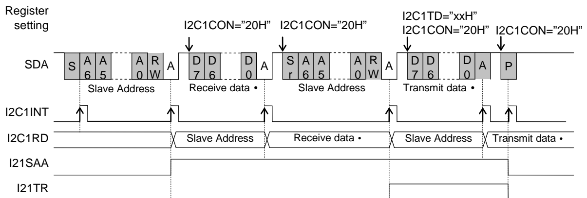
Figure 21-4 Operation Timing at Data Transmit/Receive Mode Switching
