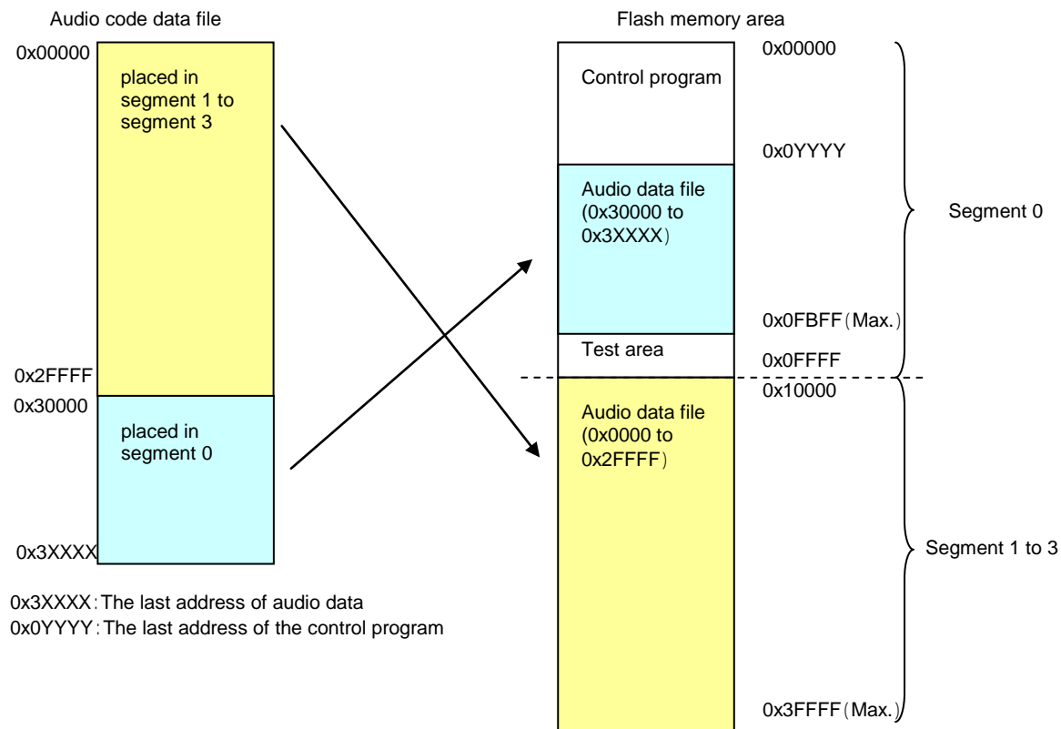
Figure 23-3 Placement of audio code data of ML610Q338/ML610Q339
