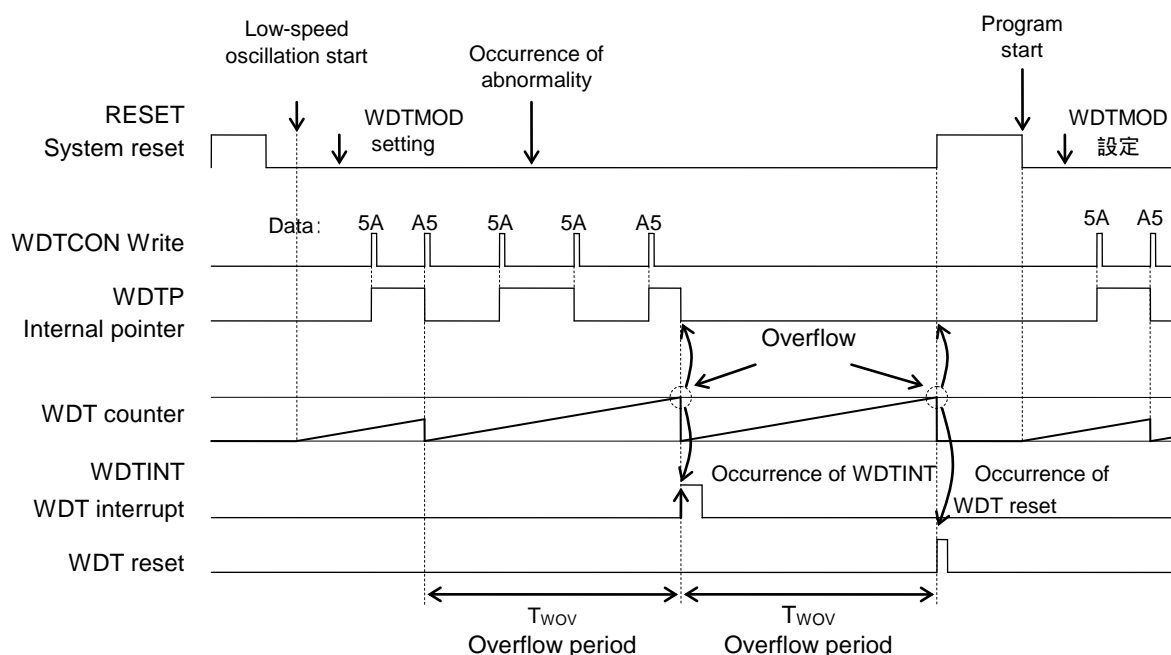
Figure 17-2 Example of Watchdog Timer Operation
