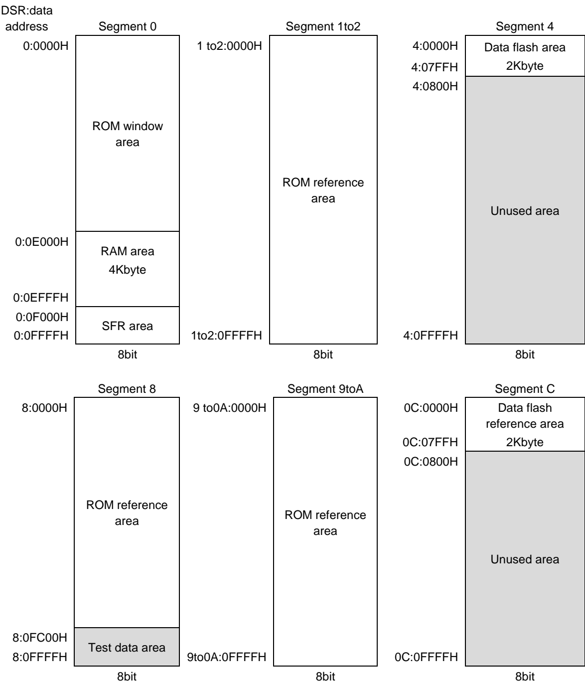
Figure 2-3 Configuration of Data Memory Space of ML610Q327
