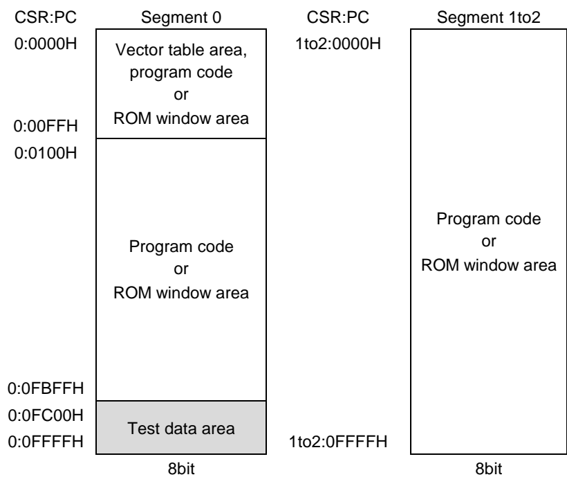
Figure 2-1 Configuration of Program Memory Space(192Kbytes) of ML610Q327
