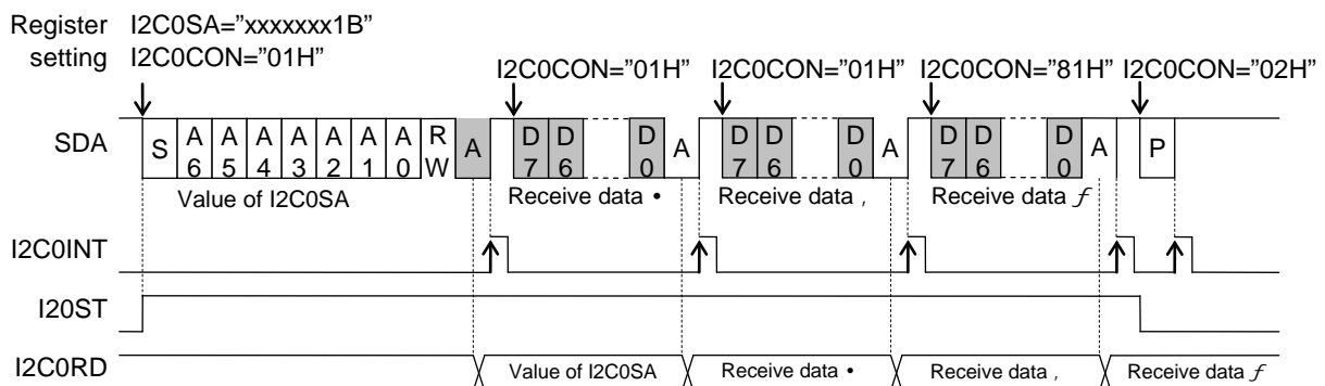
Figure 20-3 Operation Timing in Data Receive (Read)
