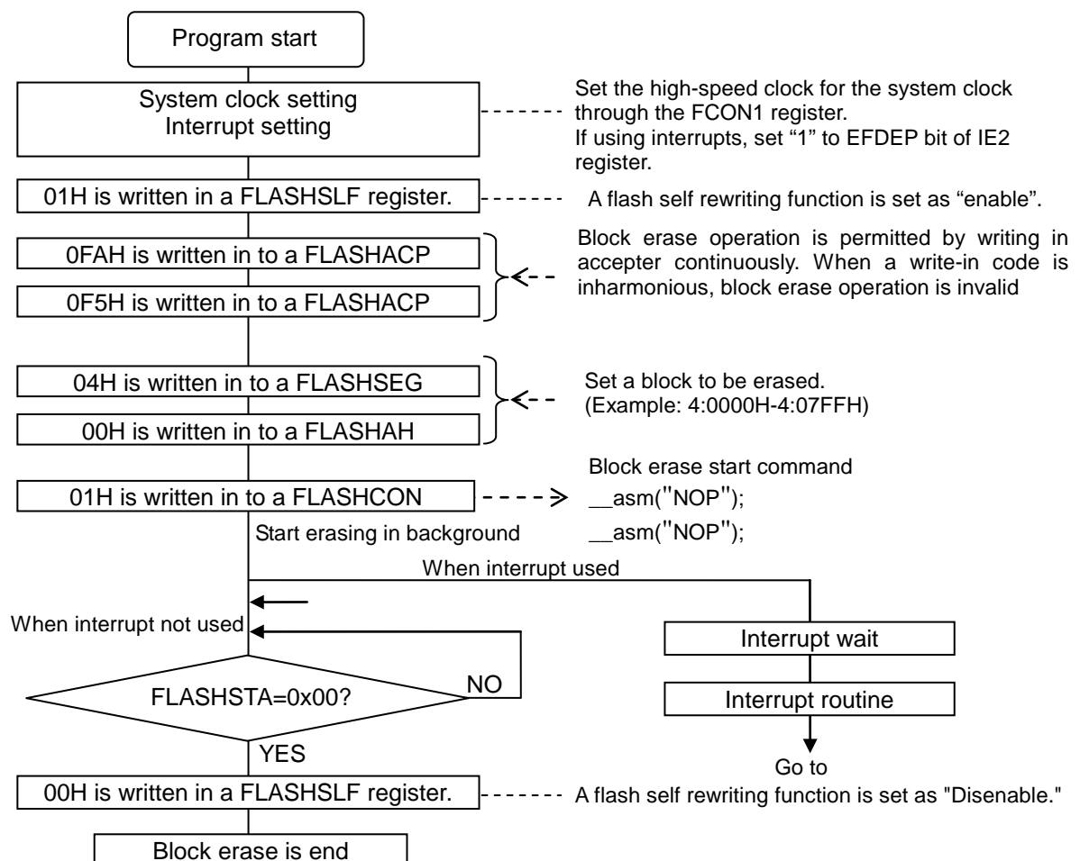
Figure 25-2 Block erase flow
