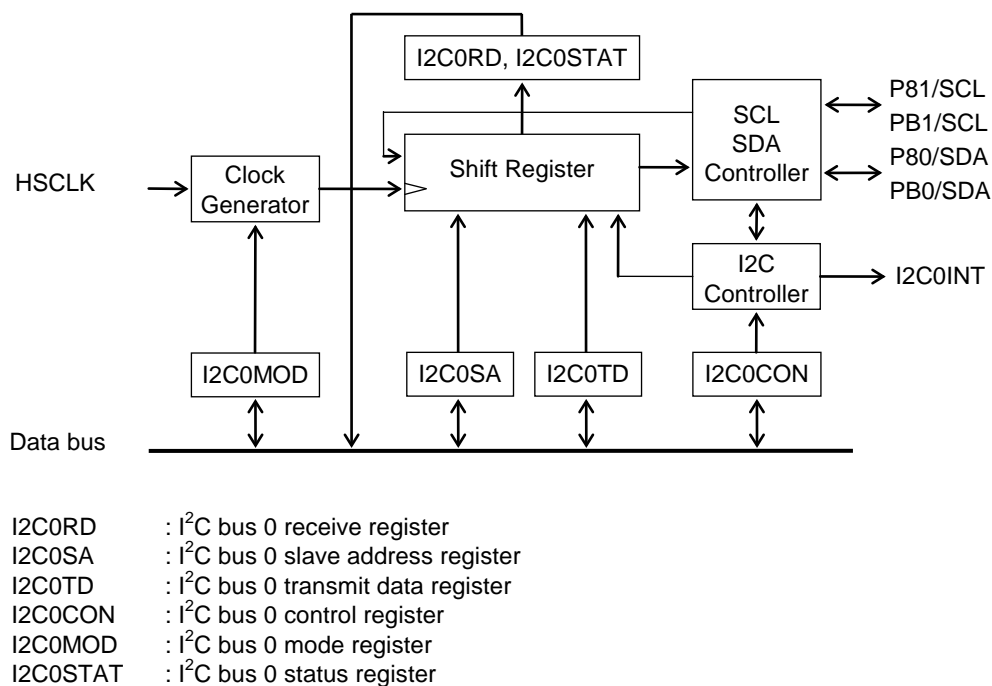
Figure 20-1 Configuration of I 2 C Bus Interface
