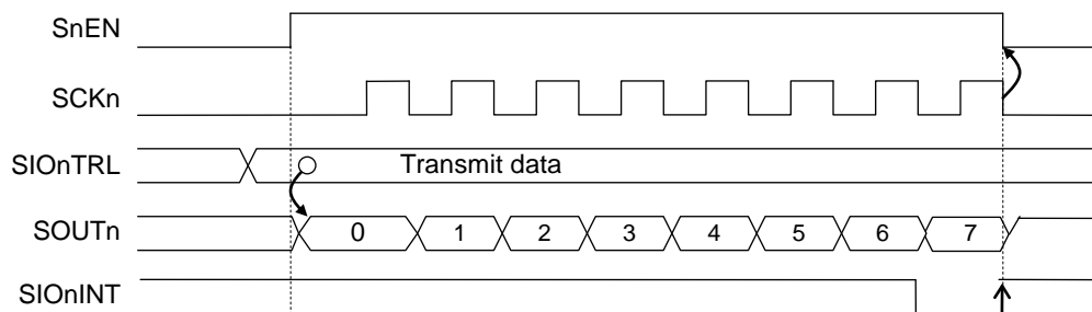
Figure 18-3 Transmit Operation Waveforms of Synchronous Serial Port n for Clock Type 1 (8-bit Length, LSB first, n=0,1)
