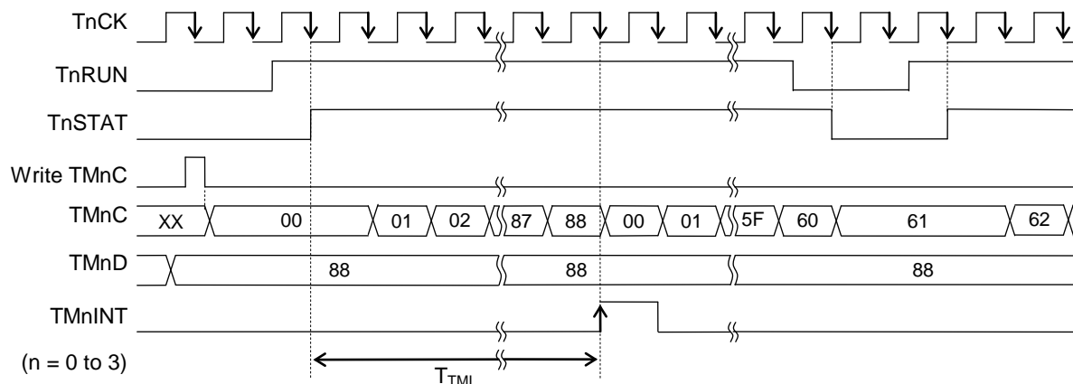
Figure 15-2 Operation Timing Diagram of Timer 0 to 3
