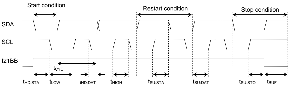
Figure 21-6 Operation Waveforms of SDA and SCL Signals and I21BB Flag
