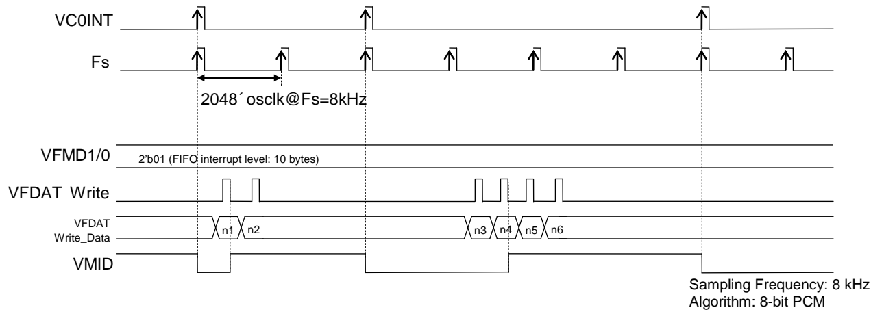
Figure 23-6 Basic Operation Timing of Audio Playback
