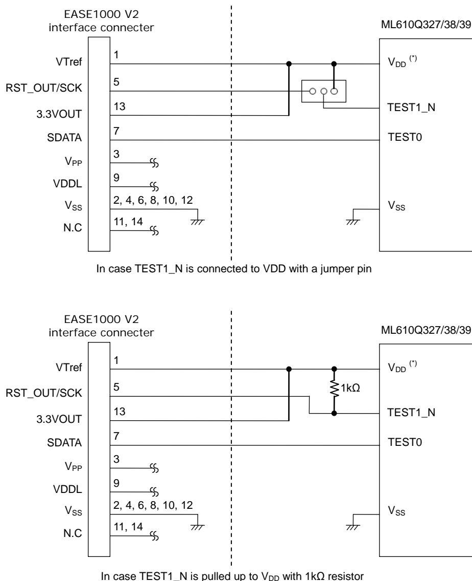
Figure 27-1 EASE1000 V2 Connections when 3.3VOUT power from EASE1000 V2 is used for V_{DD}
