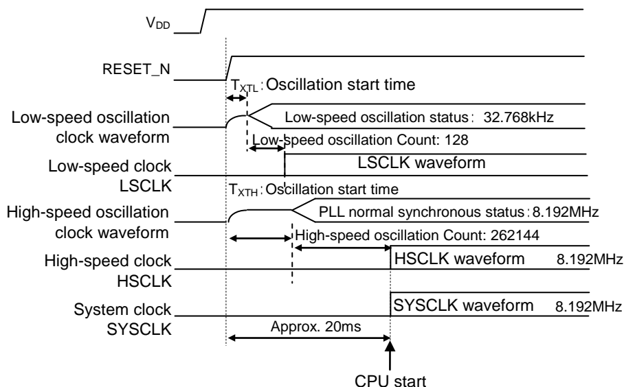
Figure 3-6 Operation of the High-Speed Clock Generation Circuit at Power-On
