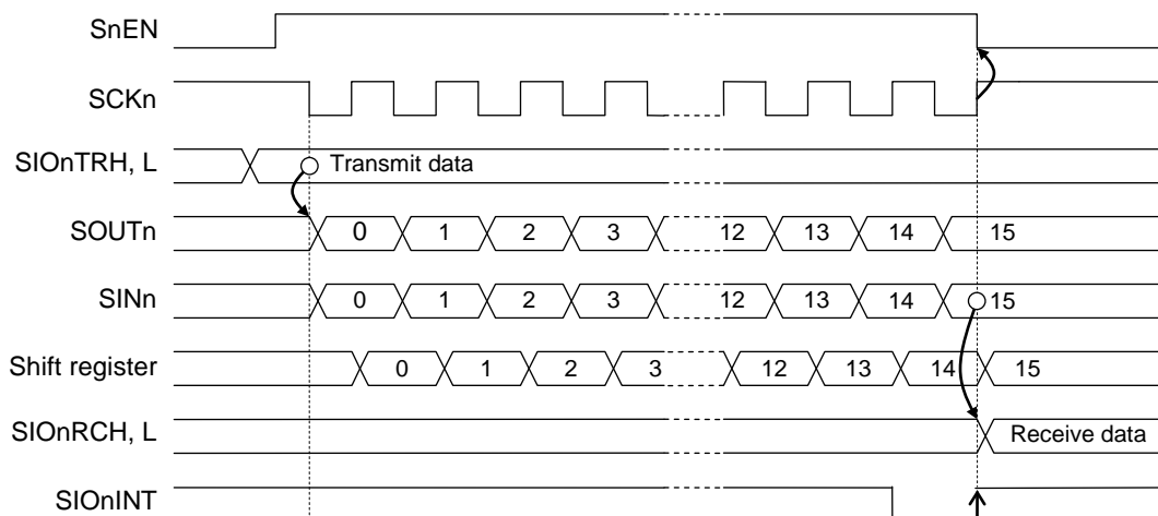
Figure 18-6 Transmit/Receive Operation Waveforms of Synchronous Serial Port n (16-bit Length, LSB first, Clock Type 0 (SPI mode 3), n=0,1)
