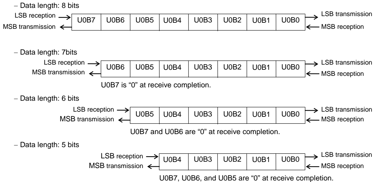
Figure 19-4 Relationship between Transmit/Receive Buffer and Transmit/Receive Data
