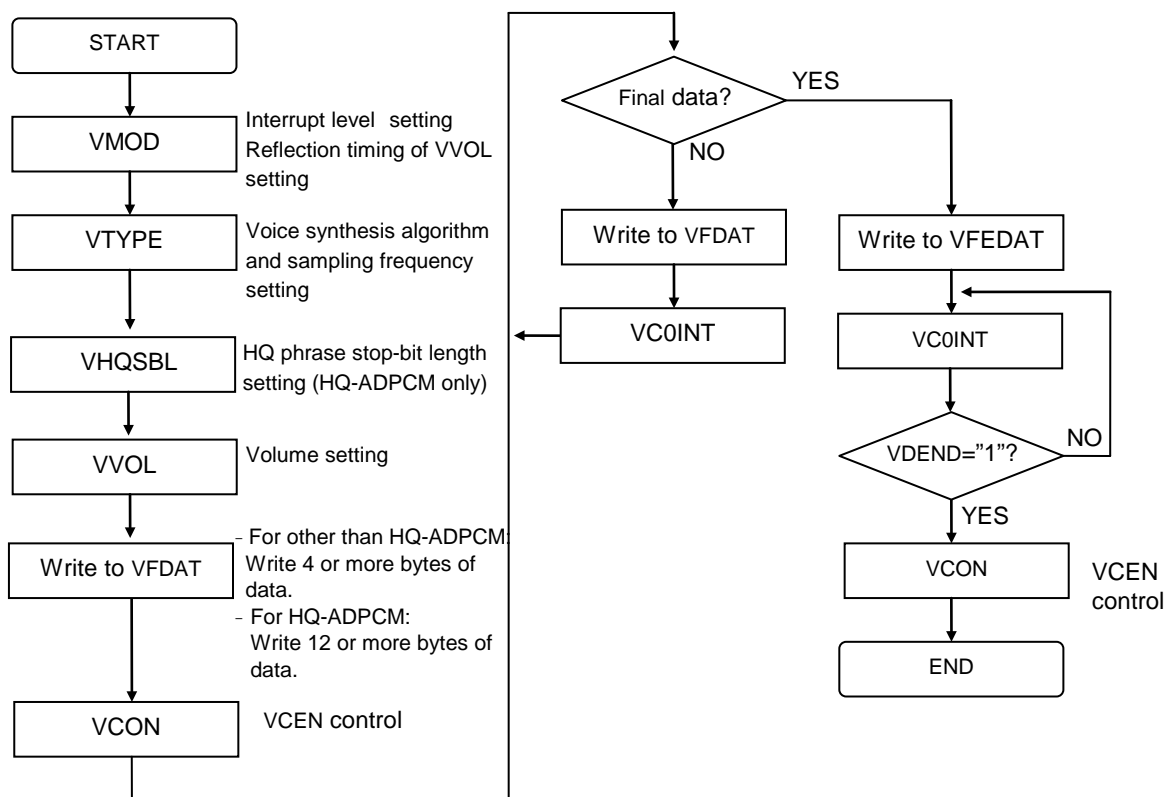
Figure 23-4 Flow of Audio Playback
