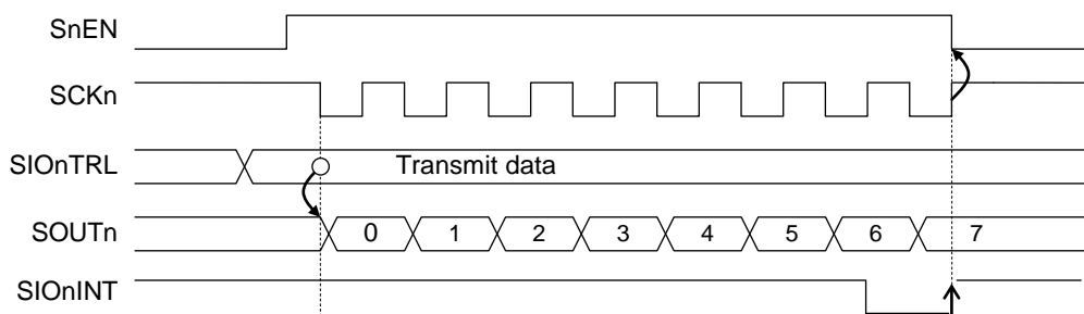
Figure 18-2 Transmit Operation Waveforms of Synchronous Serial Port n for Clock Type 0 (8-bit Length, LSB first, n=0,1)
