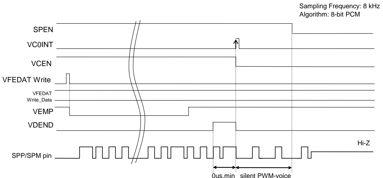
Figure 23-9 Power-Down Timing
