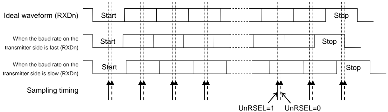
Figure 19-9 Baud Rate Errors and Reception Margin
