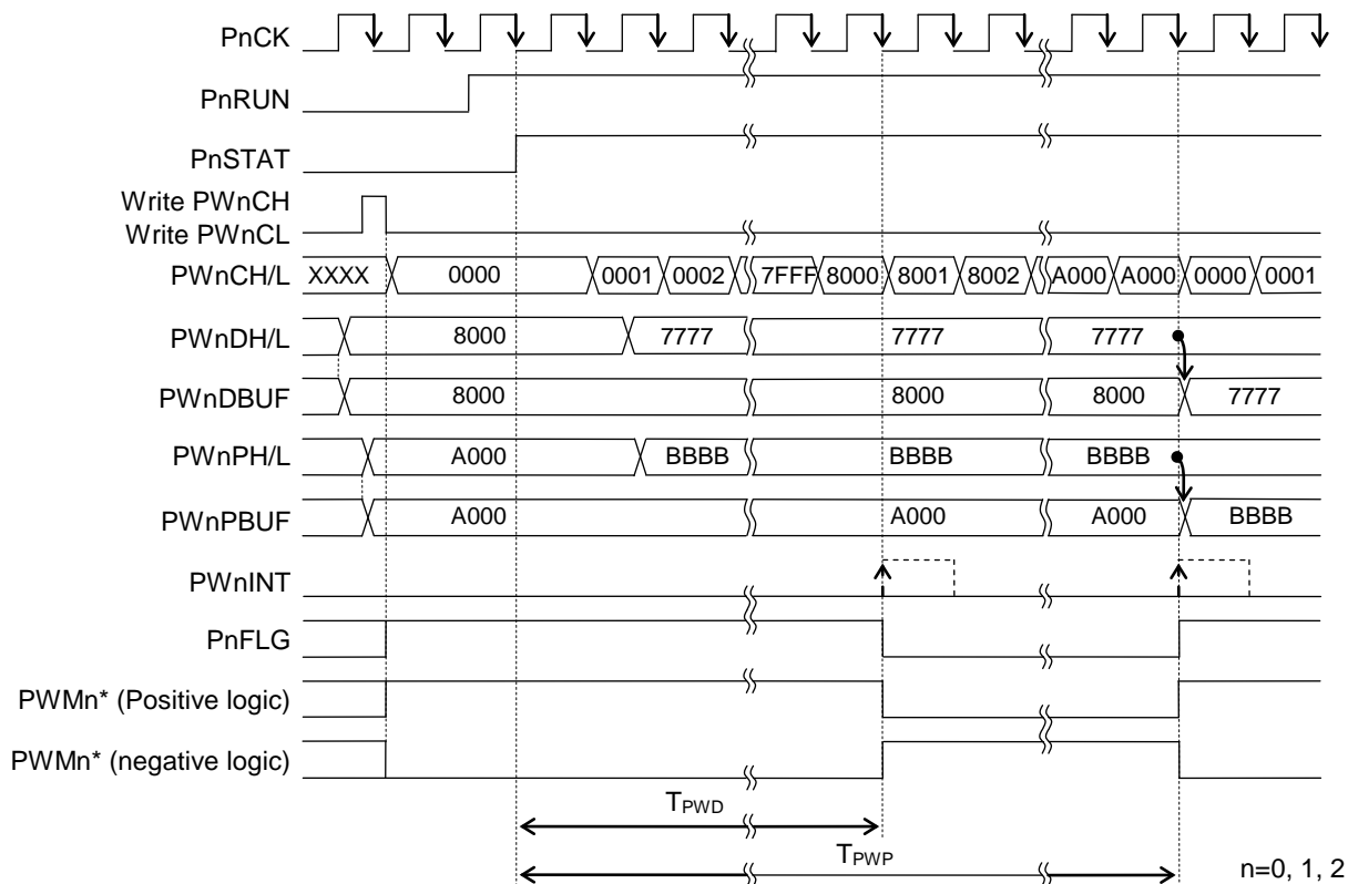
Figure 16-2 (1/2) Operation Timing Diagram of PWMn(n=0, 1, 2)
