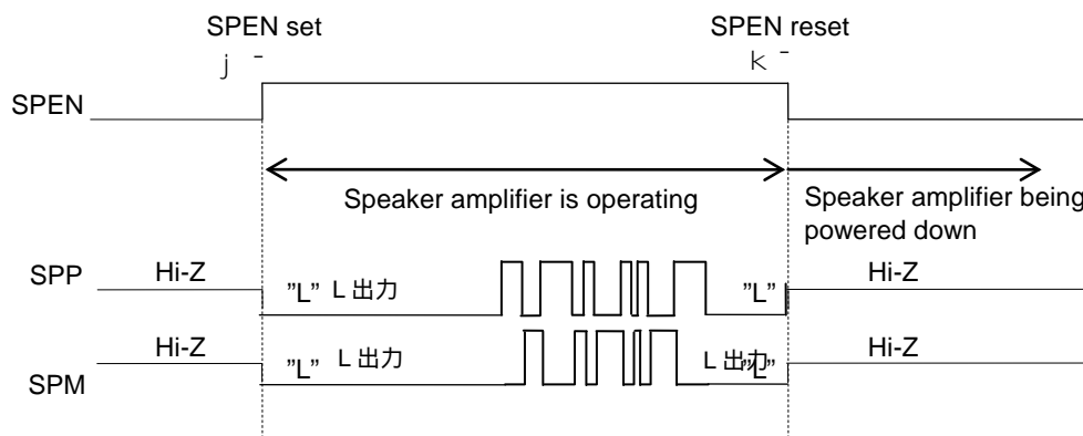
Figure 24-2 Example of Operation Timing
