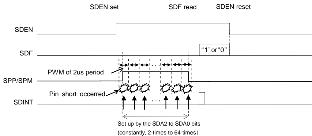
Figure 24-6 Example of Operation Timing
