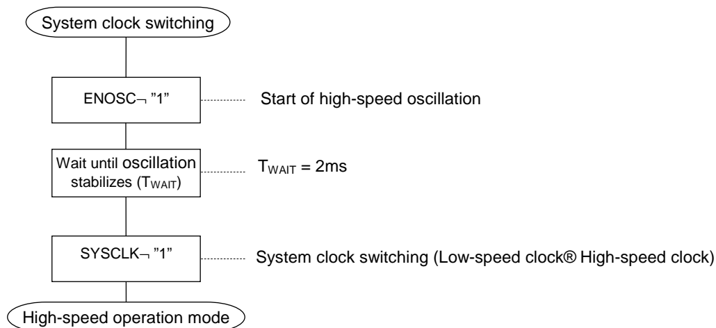
Figure 3-9 Flow of System Clock Switching Processing (LSCLK® HSCLK)
