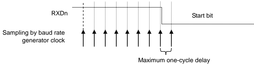
Figure 19-7 Start Bit Detection Timing (Positive Logic)
