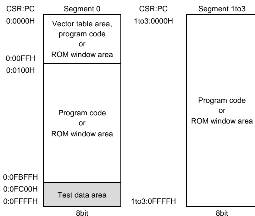
Figure 2-2 Configuration of Program Memory Space (256Kbytes) of ML610Q338/ML610Q339
