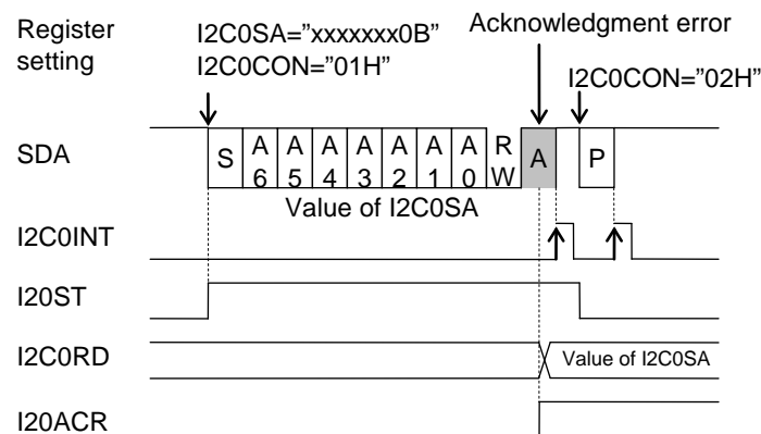
Figure 20-5 Operation Suspend Timing at Occurrence of Acknowledgment Error
