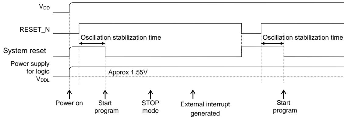
Figure 26-2 Waveforms of Power Supply Circuit Operation
