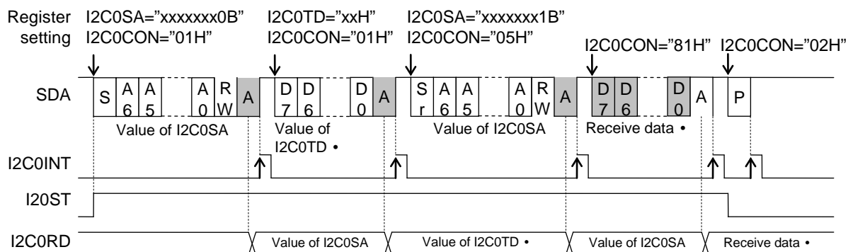
Figure 20-4 Operation Timing at Data Transmit/Receive (Write/Read) Switching
