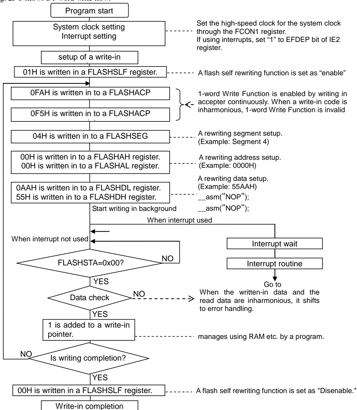
Figure 25-3 1-word Write flow
