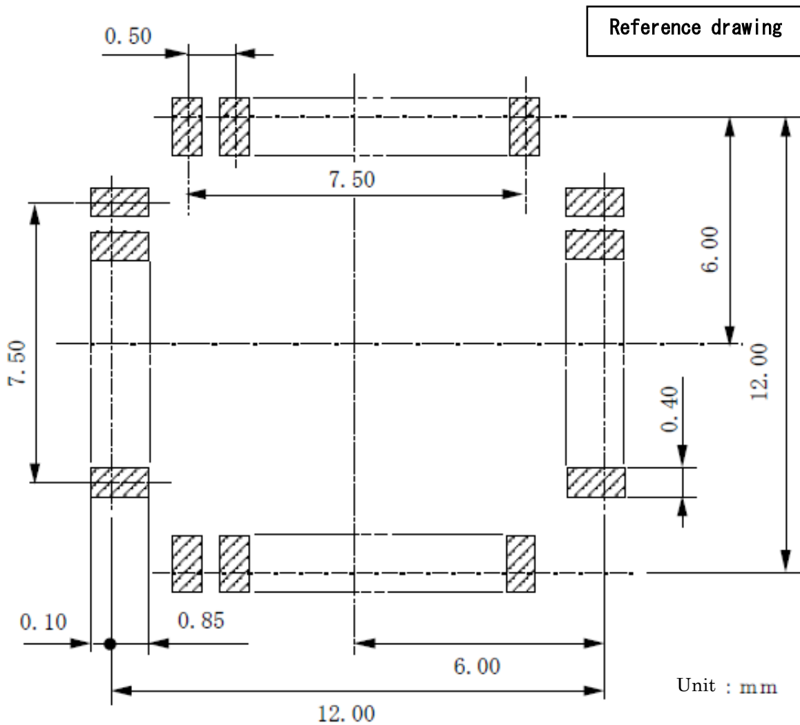
Figure of soldering department terminal existence range (64-pin TQFP)
