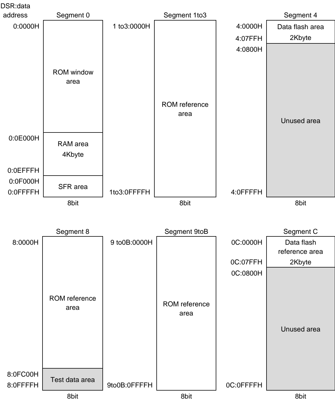
Figure 2-4 Configuration of Data Memory Space of ML610Q338/ML610Q339
