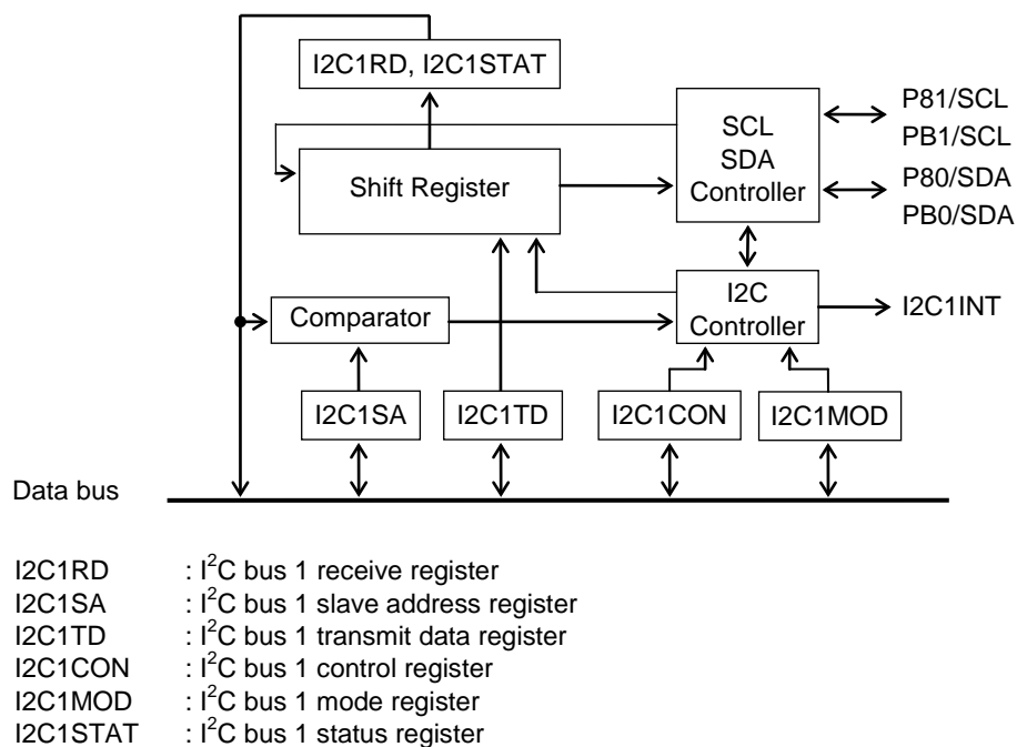
Figure 21-1 Configuration of I 2 C Bus Interface
