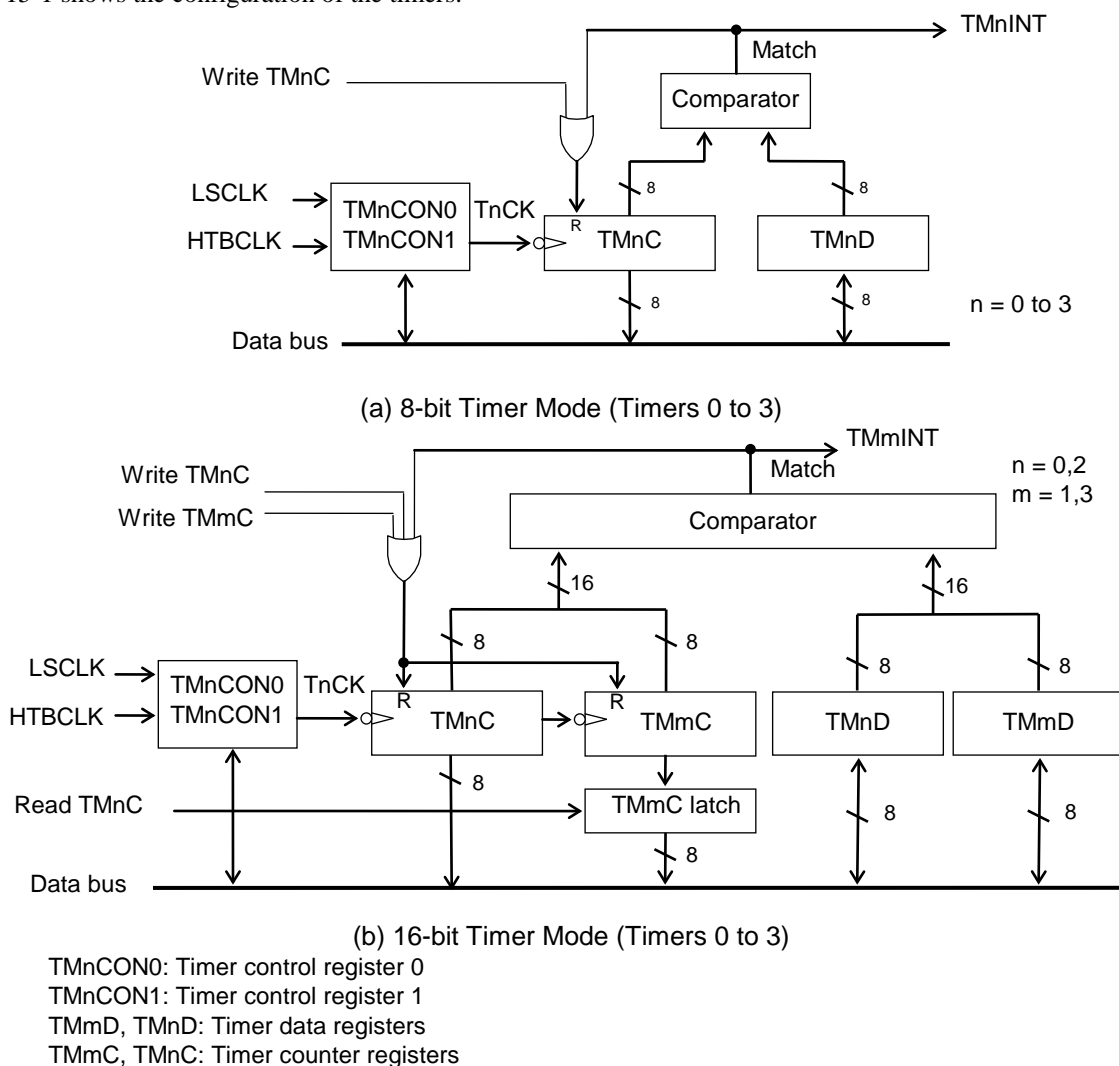
Figure 15-1 Configuration of Timers
