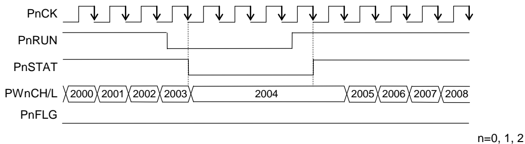
Figure 16-2 (2/2) Operation Timing Diagram of PWMn(n=0, 1, 2)
