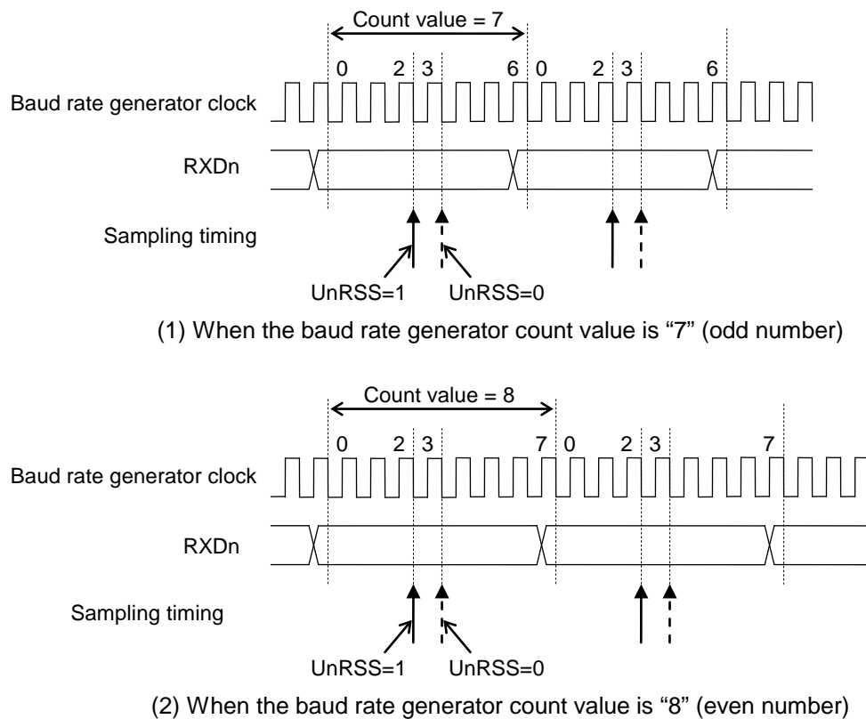
Figure 19-8 Relationship between UnRSS Bit and Sampling Timing
