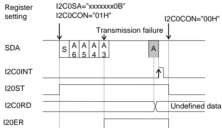
Figure 20-6 Operation Timing When Transmission Fails
