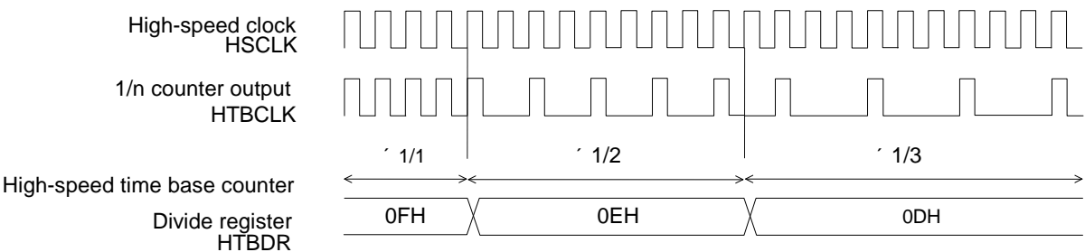
Figure 14-5 Output Waveform of HTBCLK
