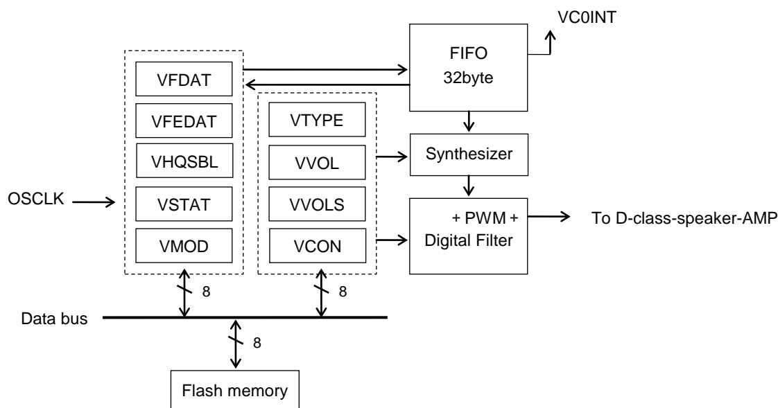
Figure 23-1 Configuration of the Audio Playback Function
