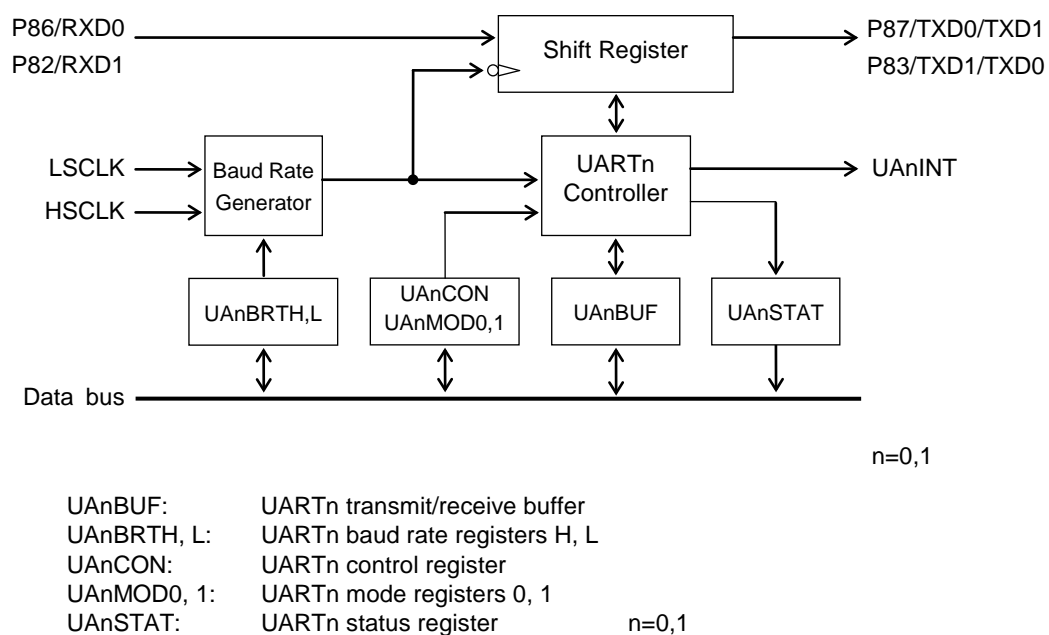
Figure 19-1 Configuration of UART
