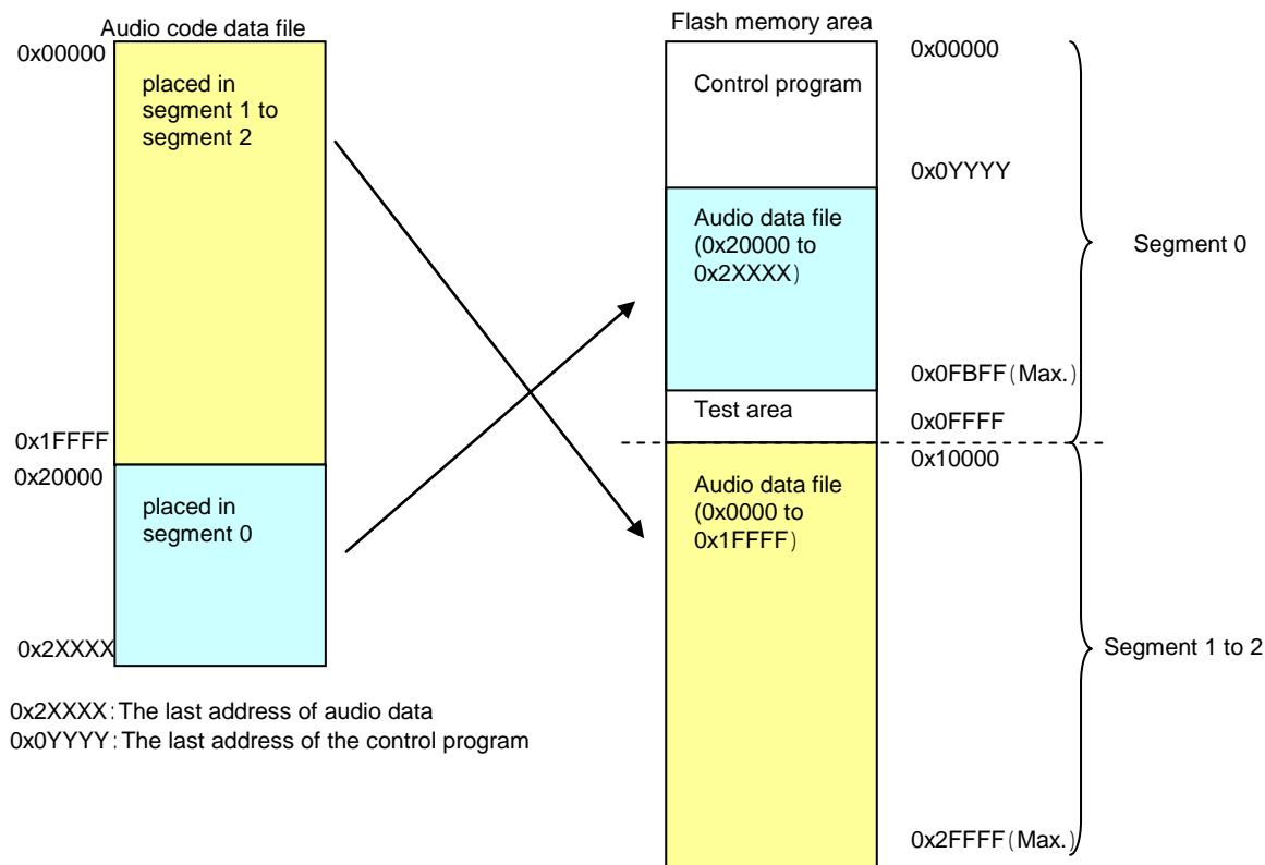
Figure 23-2 Placement of audio code data of ML610Q327
