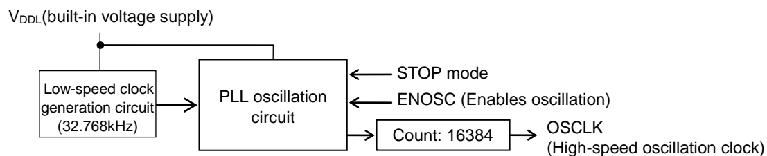
Figure 3-5 Configuration of High-Speed Clock Generation Circuit
