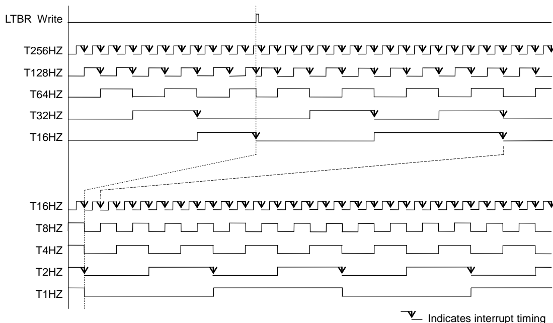
Figure 14-4 Interrupt Timing and Reset Timing by Writing to LTBR
