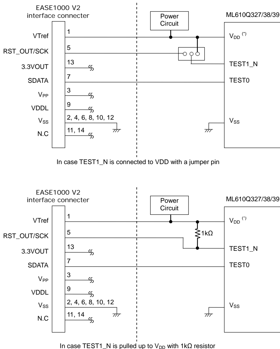
Figure 27-2 EASE1000 V2 Connections when the power from customer's power circuit is used for V DD
