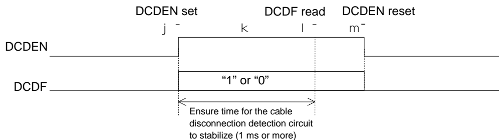
Figure 24-4 Example of Operation Timing
