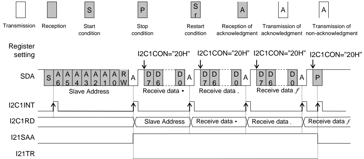
Figure 21-2 Operation Timing in Data Receive Mode
