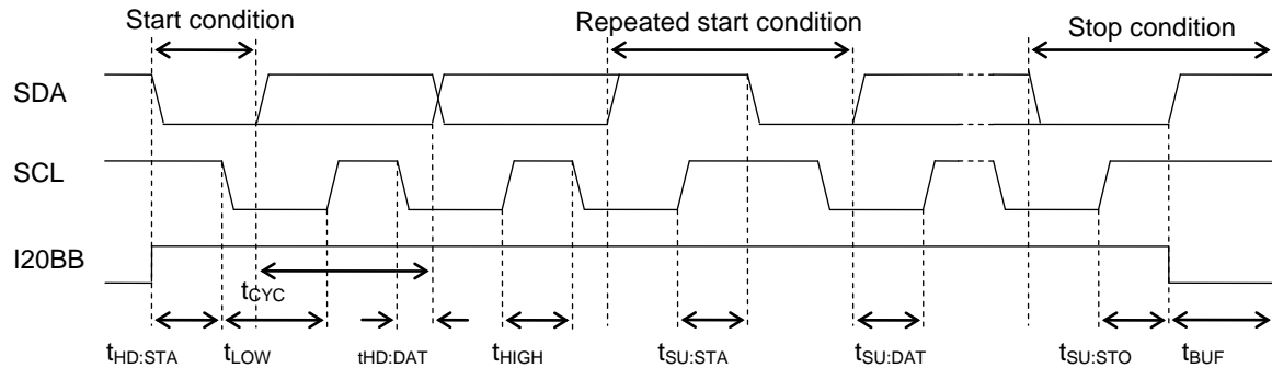
Figure 20-7 Operation Waveforms of SDA and SCL Signals and I20BB Flag
