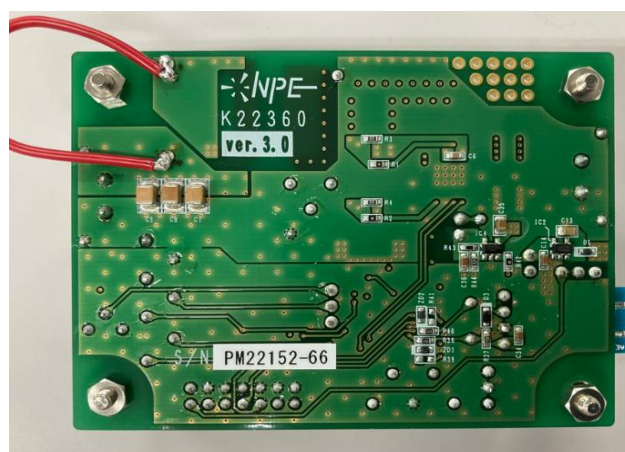
Figure 1-2. LogiCoA001-EVK-001(Bottom View)
