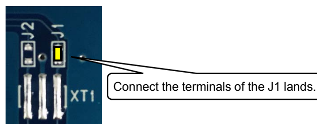
Figure 6 J1 land
