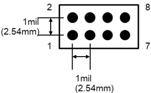
Figure 9 CN3 connectors hole pattern
