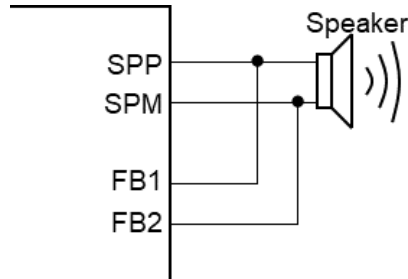
Figure 7 Connection example of FB1, FB2 pins and the SPP, SPM pins
