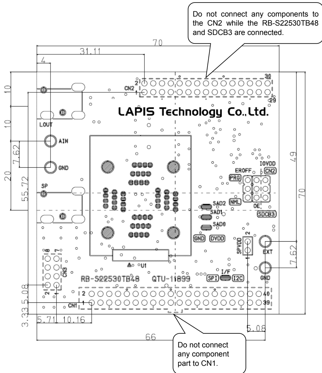
Figure 10 PCB layout
