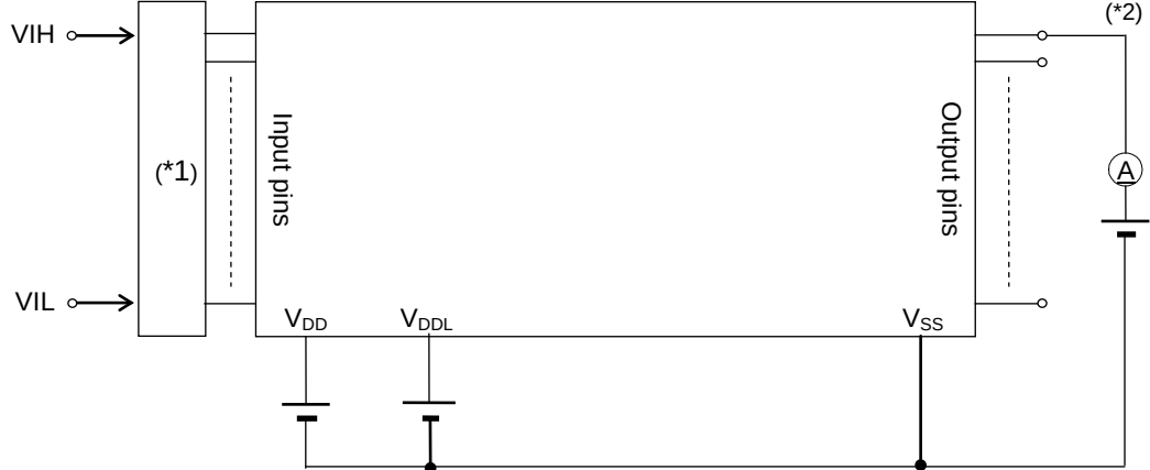
Measuring circuit 3
