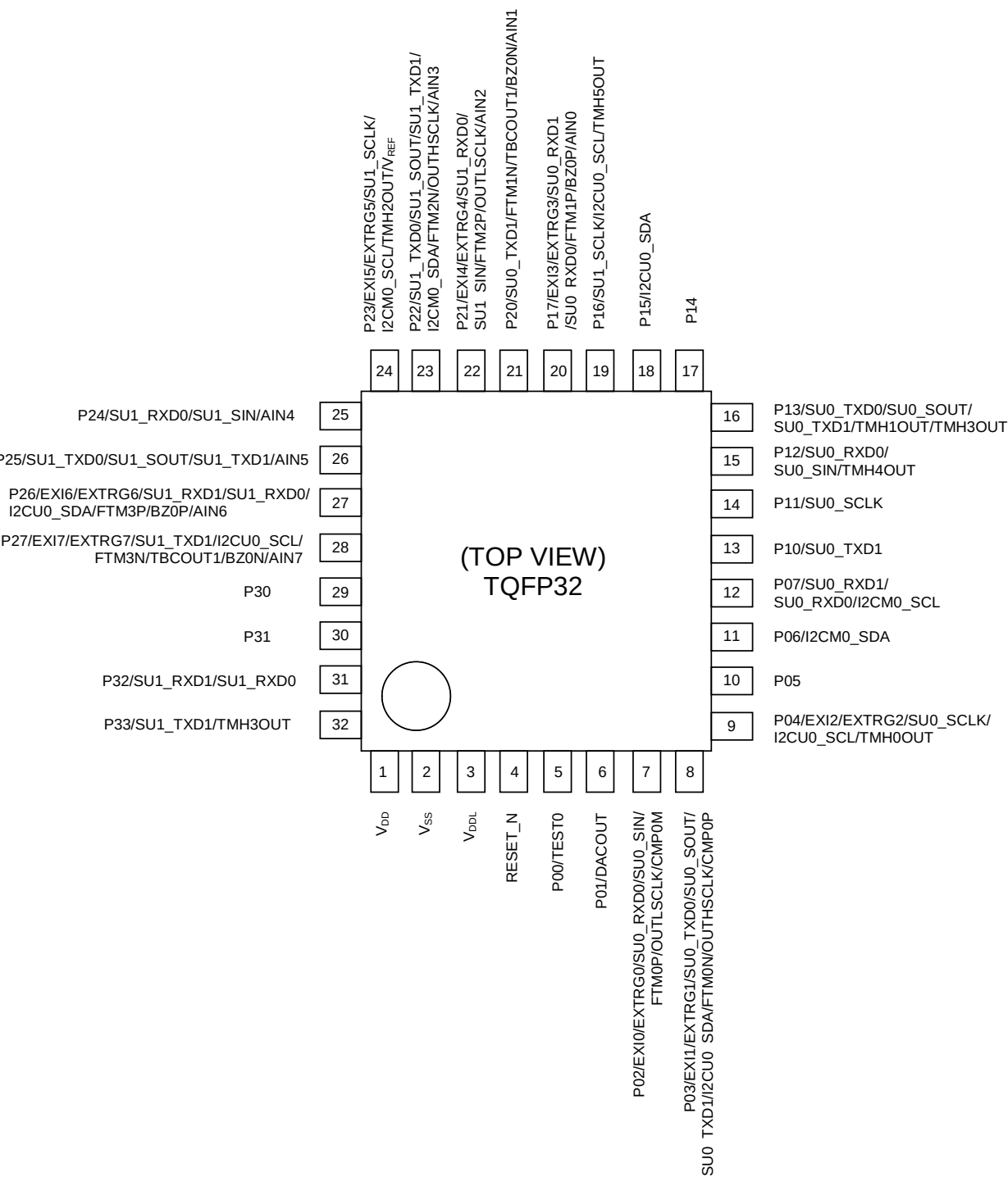
Pin Layout of ML62Q1265A/1266A/1267A 32pin TQFP Package
