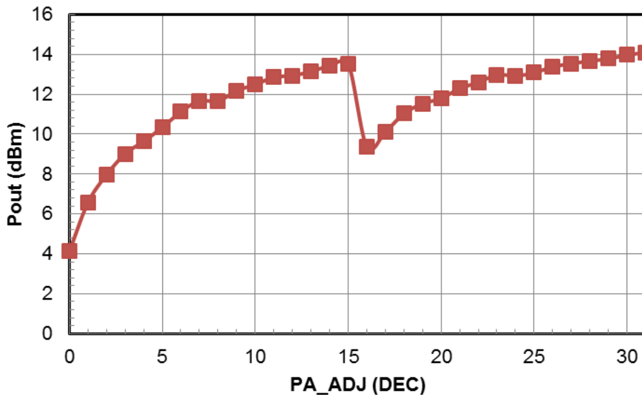
The relationship between PA_ADJ[4:0] and PA output (just for reference) (In case of 13dBm mode)
