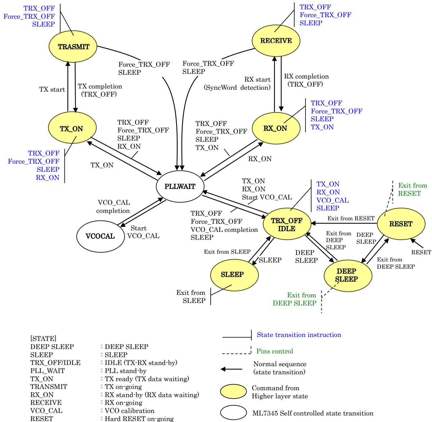
LSI state diagram
